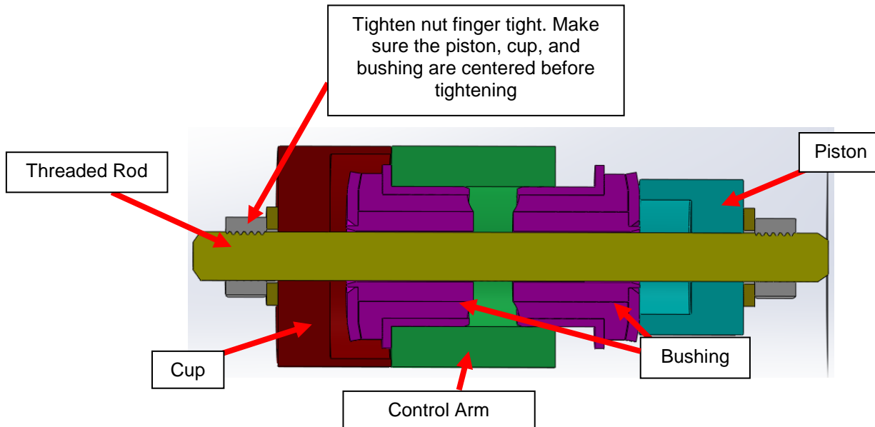
Figure 1: Installation Tool and Bushing / Upright Assembly
